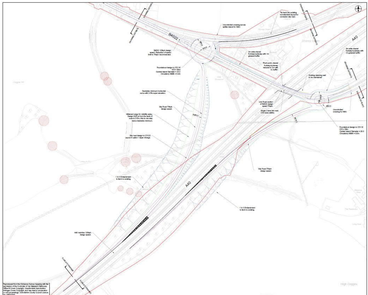
Figure 69 Option 2A-F
