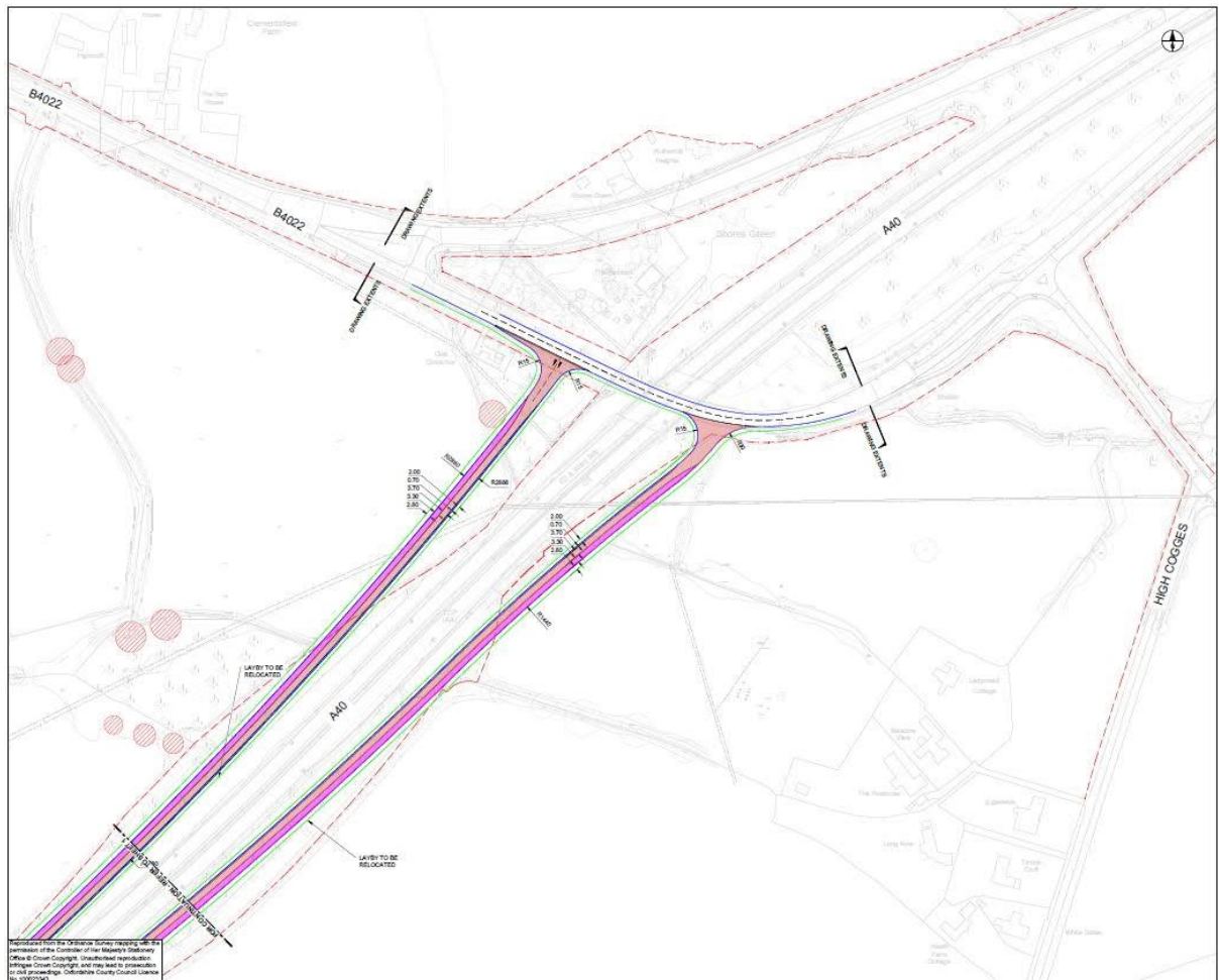
Figure 71 Option 2A-H
