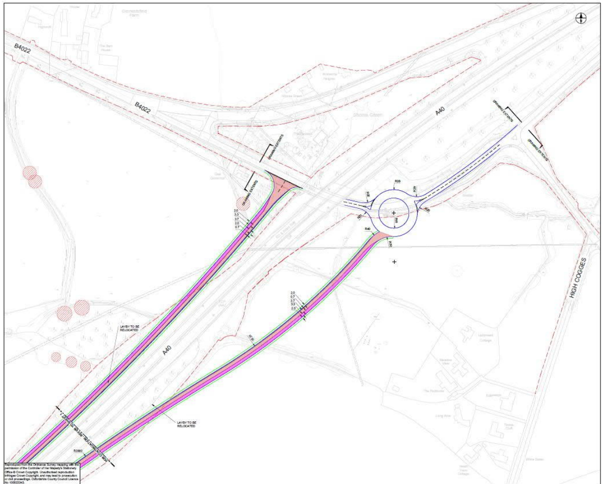
Figure 65 Option 2A-B
