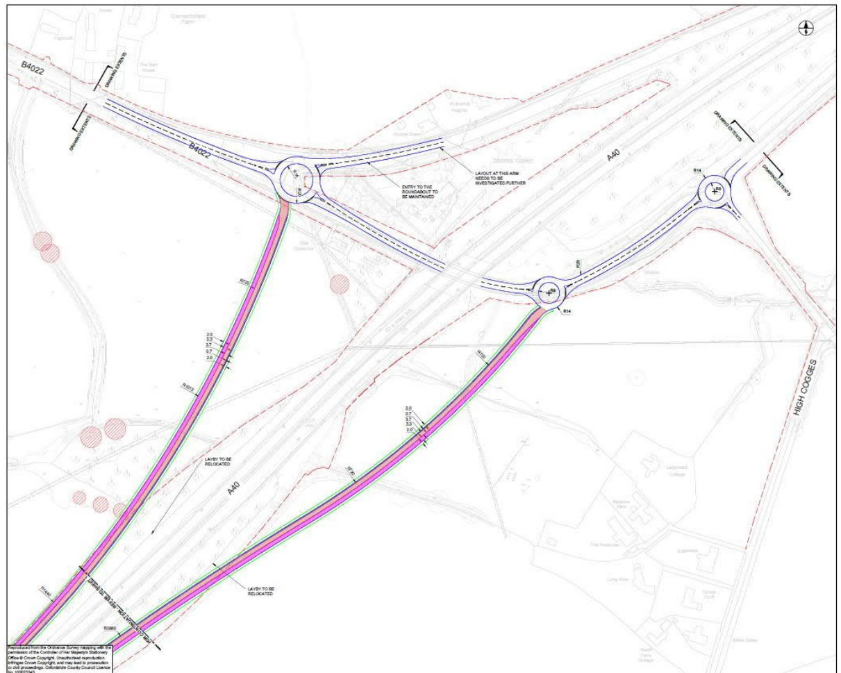
Figure 67 Option 2A-D
